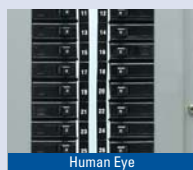
Human Eye
